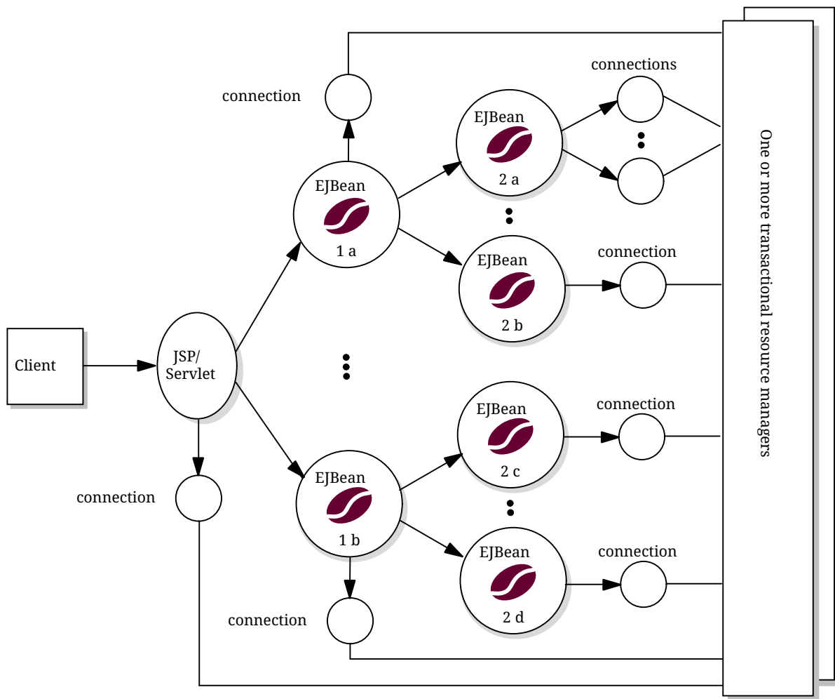
Figure 8. Servlets/Pages Accessing Enterprise Beans
