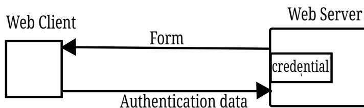
Figure 4. Initial Authentication
