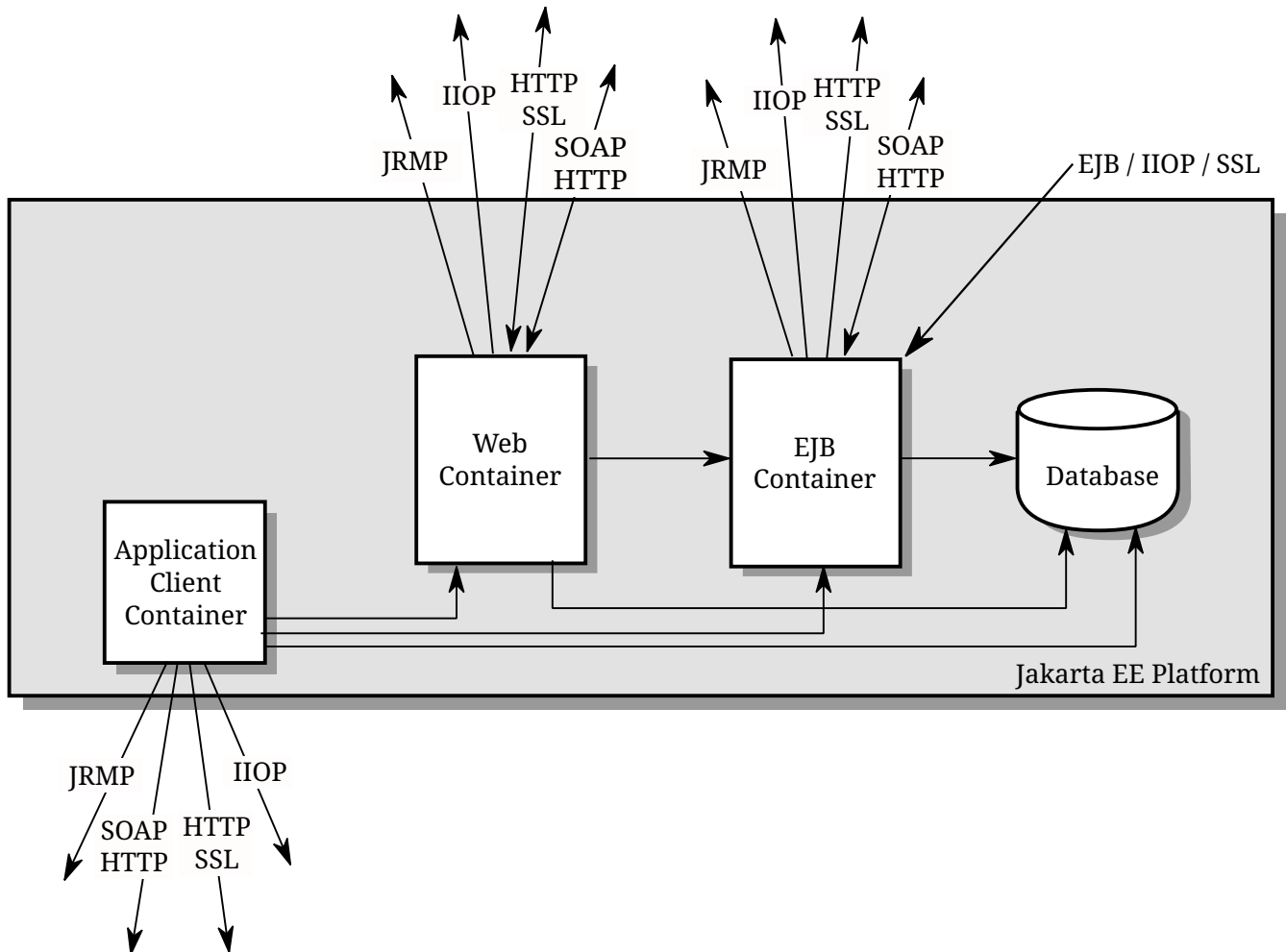
Figure 2. Jakarta EE Interoperability
