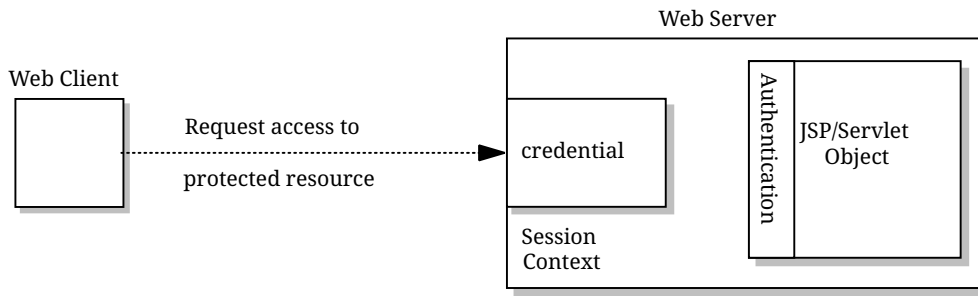
Figure 5. URL Authorization
