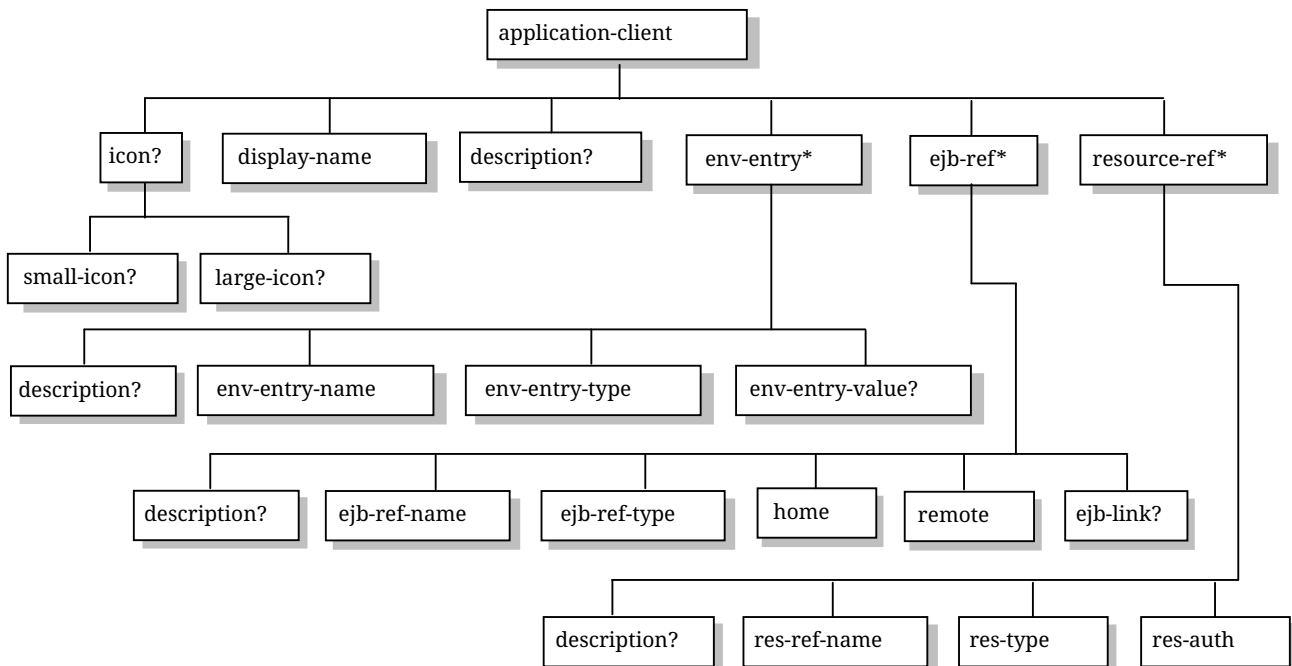
Figure 24. J2EE 1.2 application-client XML DTD Structure
